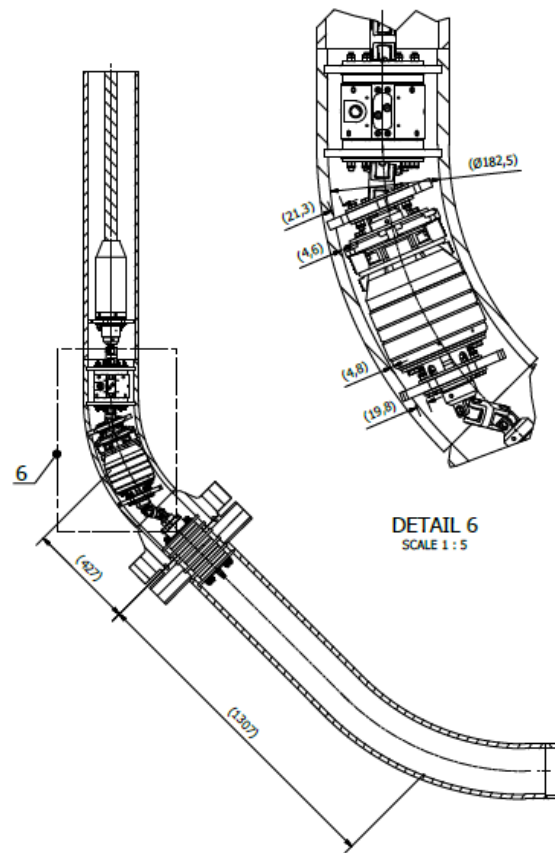
Figure 10: 8" Abandonment Plug, pigability model in 3D, 45° Bend
